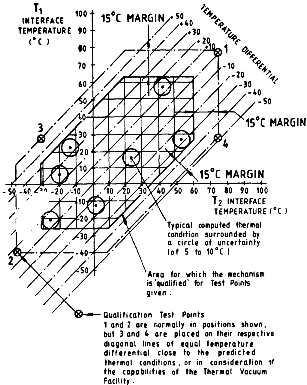
Figure 1. Example of System Used to Derive the Thermal-Gradient Test Temperatures
