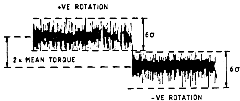
A TYPICAL TORQUE TRACE, SHOWING THE DEFINITION OF MEAN TORQUE AND TORQUE NOISE ( 6\sigma )
