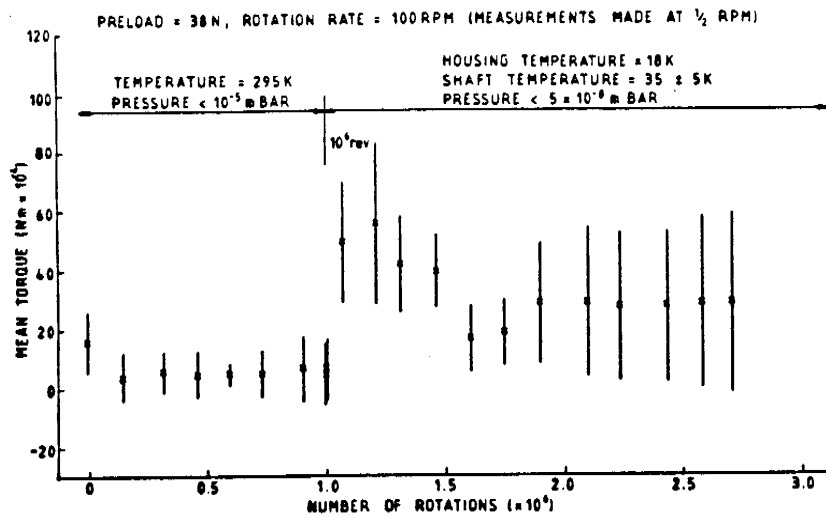
THE TORQUE PROFILE OF \text{MoS}_2 / DUROID - LUBRICATED BEARINGS
