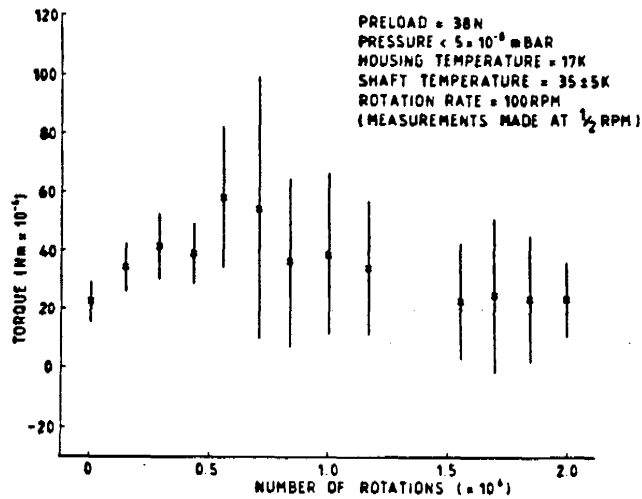
THE TORQUE PROFILE OF DUROID-LUBRICATED BEARINGS OPERATING AT 19K
