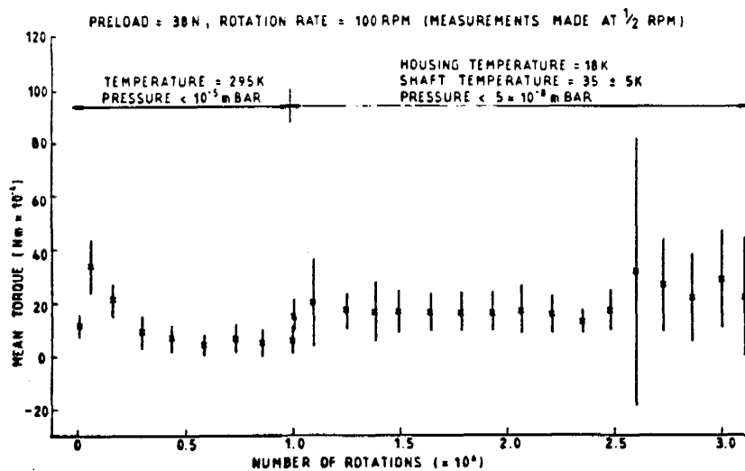
THE TORQUE PROFILE OF DURIOD-LUBRICATED BEARINGS OPERATING AT 295 K AND AT 18 K
