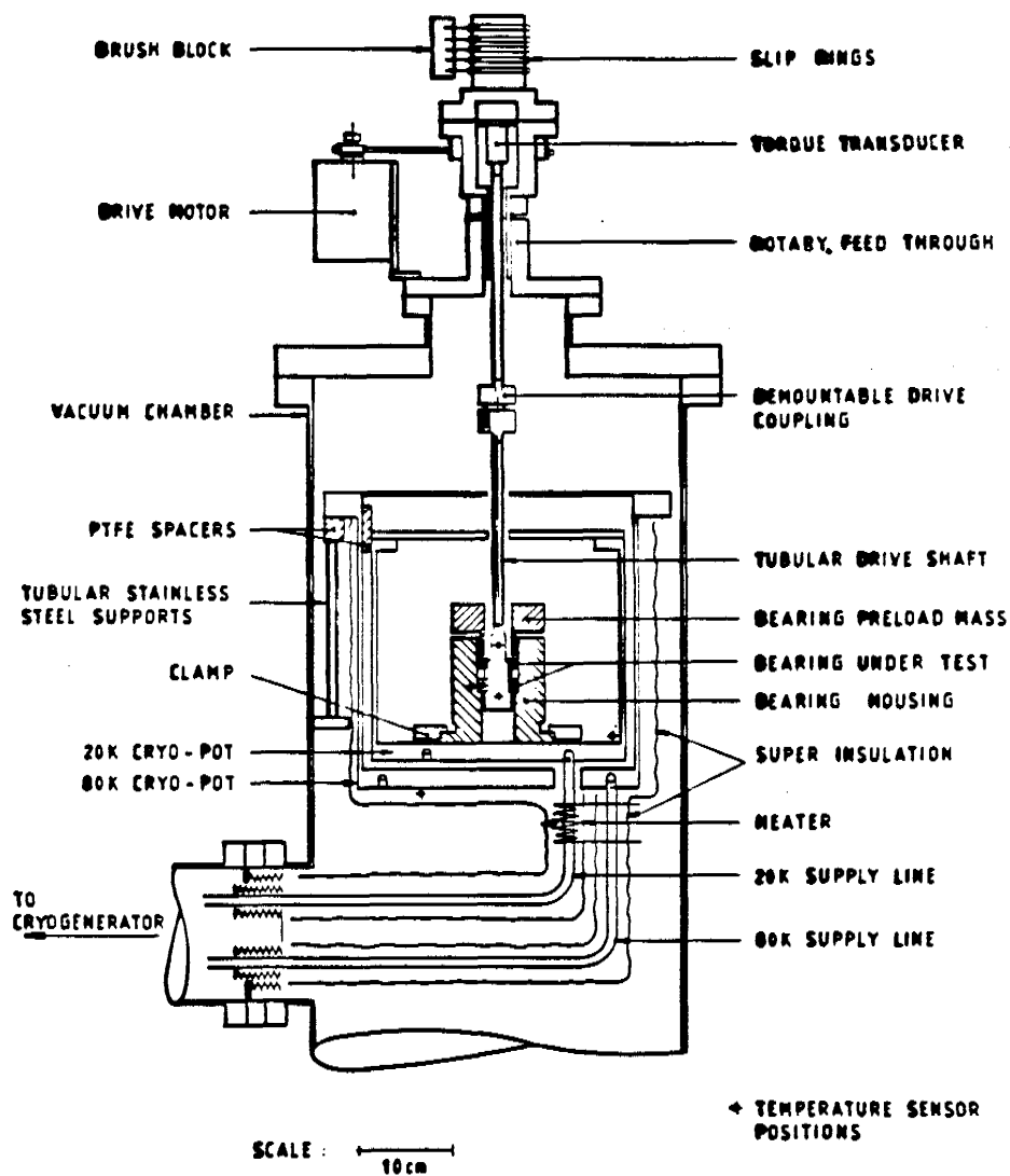
SCHEMATIC OF THE CRYOGENIC VACUUM CHAMBER AND BALL BEARING TEST APPARATUS
