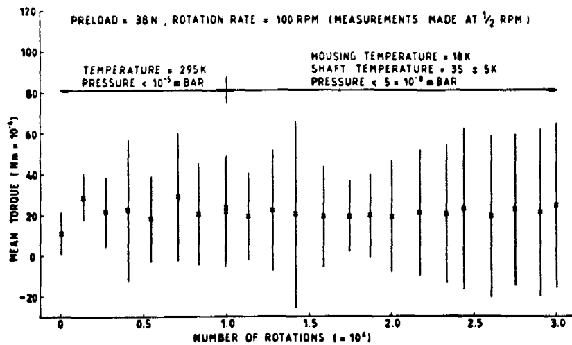
THE TORQUE PROFILE OF LEAD-LUBRICATED BEARINGS OPERATING AT 295K AND AT 18K
