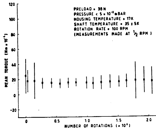
THE TORQUE PROFILE OF LEAD-LUBRICATED BEARINGS OPERATING AT 17K
