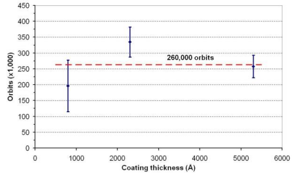
Figure 12. Lifetimes of MoS 2 as a function of coating thickness
