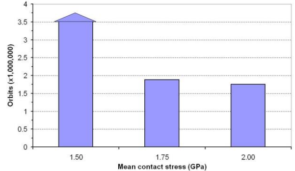
Figure 14. Lifetimes of lead as a function of mean contact stress
