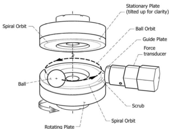
Figure 1. Internal arrangement of SOT, showing flat and guide plates
