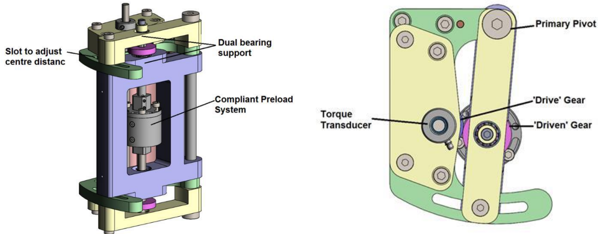
Figure 7. Conventional gear test setup for ESTL's miniature gear/pinion testing rig
