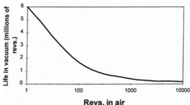
Figure 1. Low-torque life of MoS 2 lubricated ED20 bearings in vacuum as a function of in-air operation prior to vacuum testing [4]
