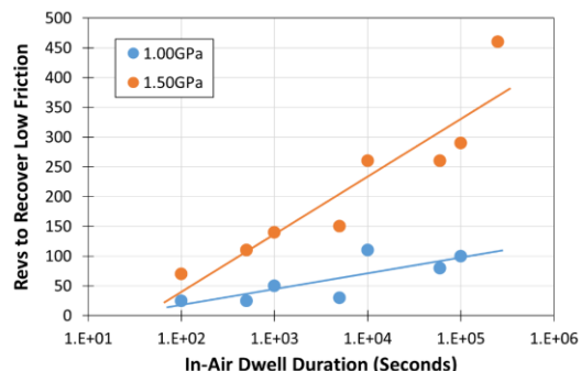
Figure 2. PoD revs required to achieve low friction performance of sputtered MoS 2 under vacuum following moist air dwell period [6]
