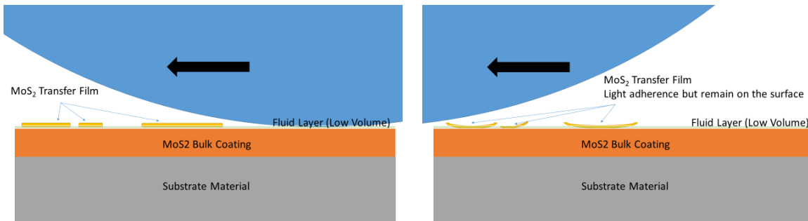
Figure 10. MoS 2 transfer film formation (3 rd body) of low fluid volume hybrid lubrication
