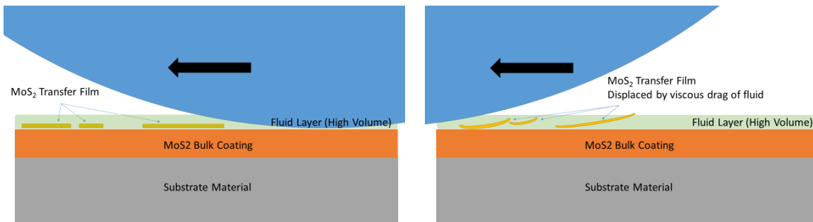
Figure 9. MoS 2 transfer film formation (3 rd body) of high fluid volume hybrid lubrication
