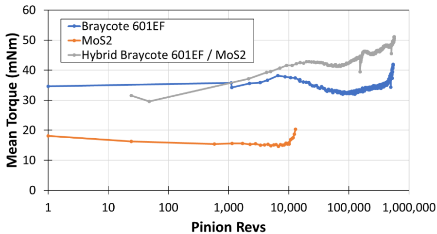
Figure 8. Mean torque behaviour of spur gear tests (parasitic torques removed)
