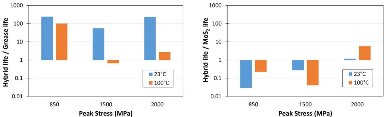
Figure 5. Hybrid Braycote 601EF/MoS 2 lifetimes as a factor of Braycote 601EF-only (left) and sputtered MoS 2 only (right) lifetimes
