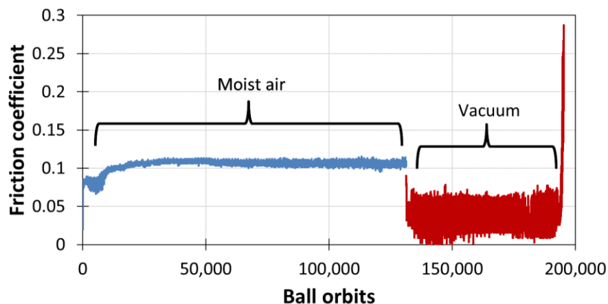
Figure 3. Hybrid Z25/MoS 2 rolling in air (blue) and vacuum (red). Elevated frictional noise during vacuum running is an artefact introduced by the analysis software and is not real
