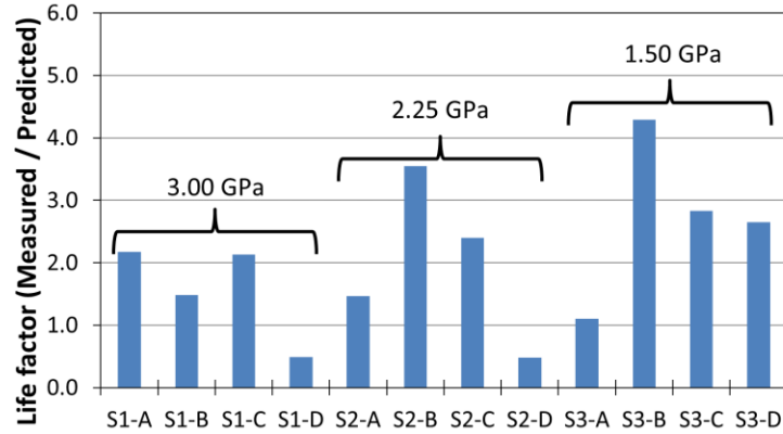
Figure 4. Measured lifetimes of hybrid Z25/MoS 2 lubrication as factor of predicted life
