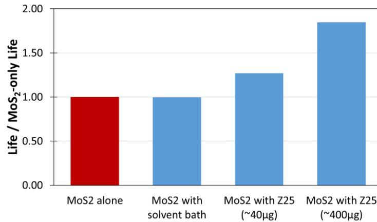
Figure 6. Normalised performance of Z25/MoS 2 lubrication under vacuum
