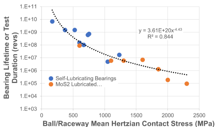
Figure 18. In vacuum bearing life or test duration v ball/raceway Hertzian contact stress for MoS 2 films and self-lubricating bearings
