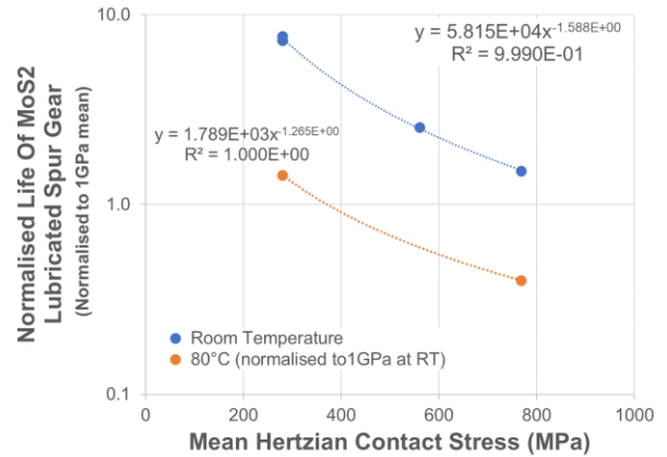
Figure 6. Normalised in vacuum lifetime of sputtered MoS 2 lubricated spur gears [19]
