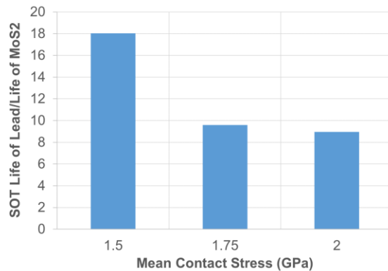
Figure 8. Relative lifetime of sputtered lead as compared to sputtered MoS 2 in vacuum (~1μm) as function of contact stress
