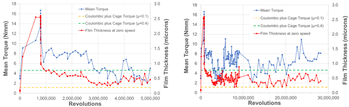
Figure 19. Type 7004 Bearing mean torque and PGM-HT film thickness v revolutions in vacuum
