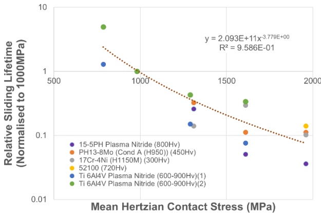
Figure 5. Normalised in vacuum lifetimes of sputtered MoS 2 in PoD test on various substrates [18]
