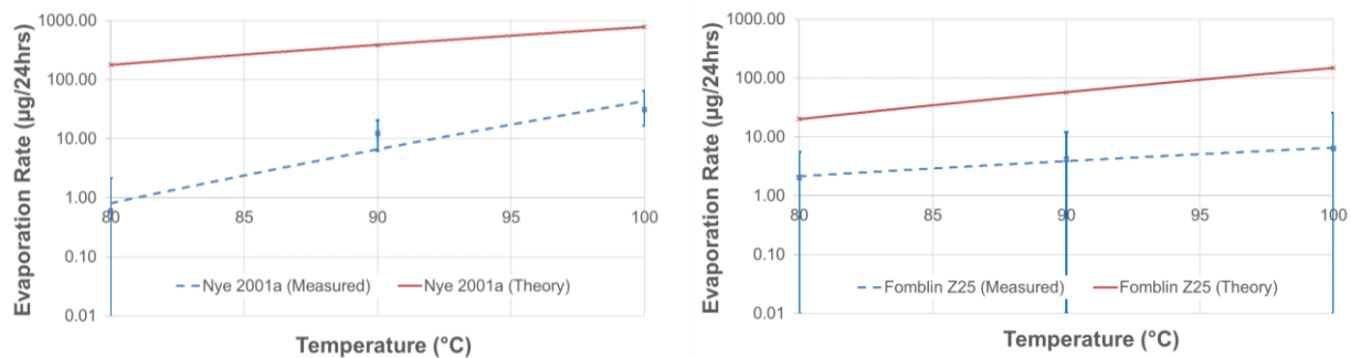
Figure 2. Comparison of experimentally measured evaporative loss rates for Nye 2001A (left) and Fomblin Z25 (right) with the predictions of Langmuir theory [11]
