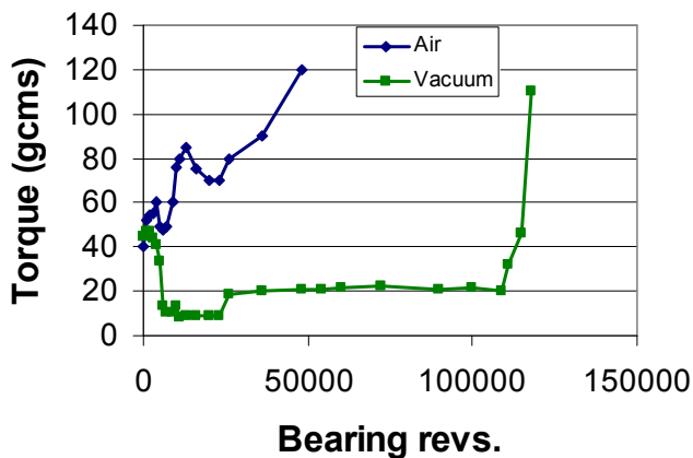
Figure 12: Bearing torque test results in air and in vacuum
