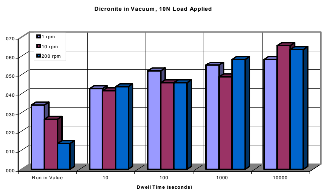
Figure 10: Effect of dwell time on Dicronite friction (in vacuum)
