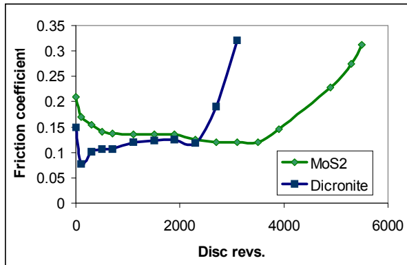
Figure 6: Pin-on disc data for Dicronite in air (corresponding data for sputtered MoS 2 is also shown)
