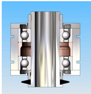
Figure 11: Ball bearing test set-up
