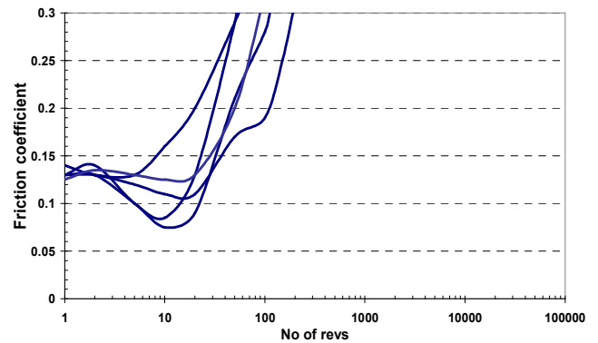
Figure 3: Test results – Supplier C (dry nitrogen)
