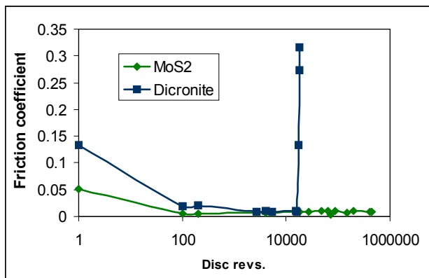
Figure 7: Pin-on disc data for Dicronite in vacuum, compared with sputtered MoS 2
