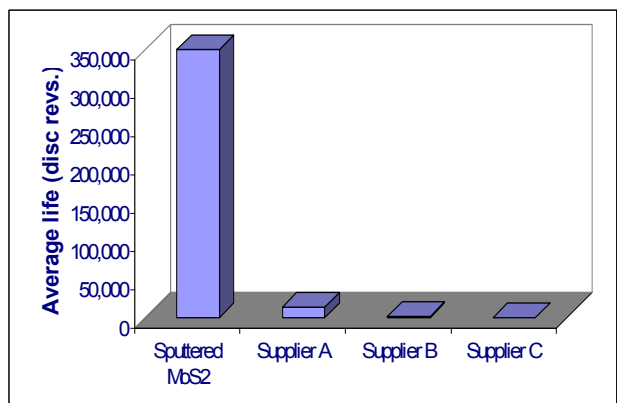
Figure 5: Comparison with sputtered MoS 2
