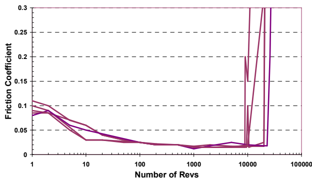
Figure 1: Test results – Supplier A (dry nitrogen)
