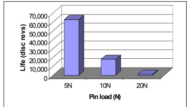
Figure 8: Effect of load on Dicronite film durabilities (in vacuum)
