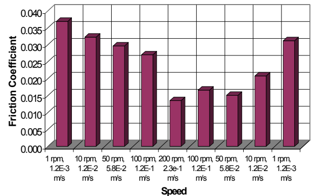
Figure 9: Effect of speed on friction coefficient of Dicronite films (in vacuum)
