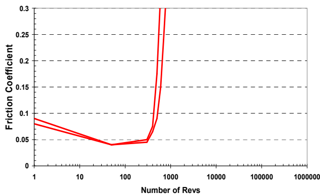
Figure 2: Test results – Supplier B (dry nitrogen)
