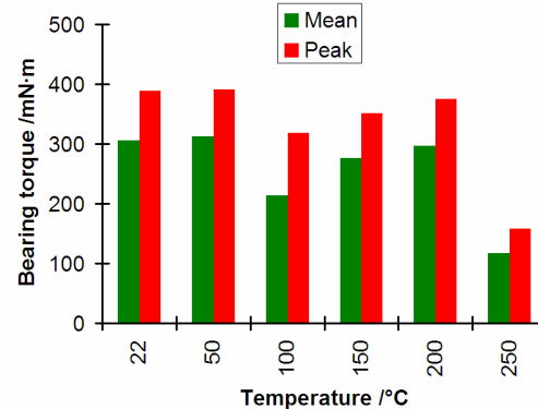
Figure 3 Results of initial tests of lead lubricated bearing with leaded bronze cages.
