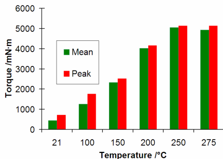
(a) Initial torque variation with temperature
