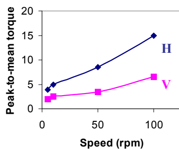
Figure 11. Torque noise variation with speed
