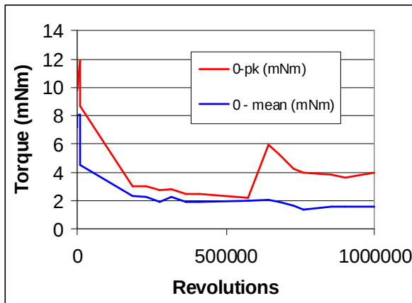
Figure 12. Test 24 results, with MoS 2 -coated bearings
