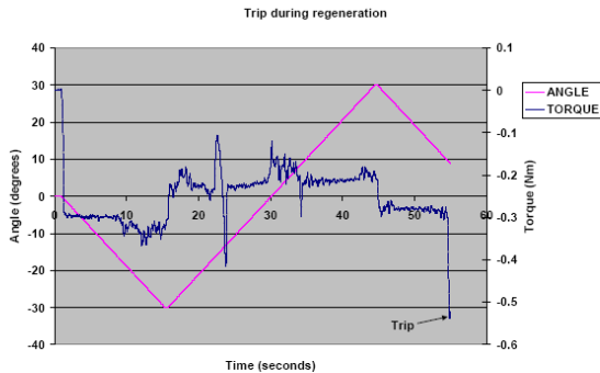
Figure 9: Trip during regeneration at 136,066 cycles (oil-lubricated ball bearings). Transient at approx -15 deg attributable to presence of hard particle in the bearing.
