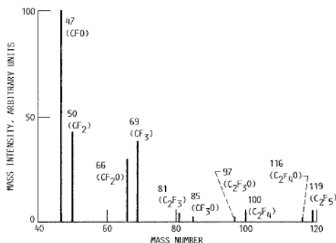
Figure 17: Mass spectrum of gaseous species evolved during testing Fomblin Z25 against 440C steel[2]
