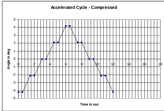
Figure 1: Life test profile
