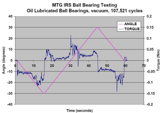
Figure 4: Regeneration profile for oil lubricated ball bearings in vacuum (107,521 cycles)
