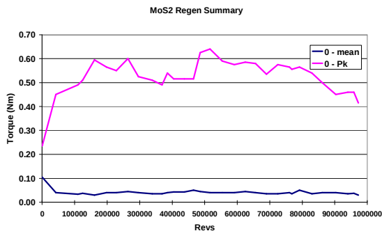
Figure 5: Summary of mean and 0-peak torques during regeneration cycles
