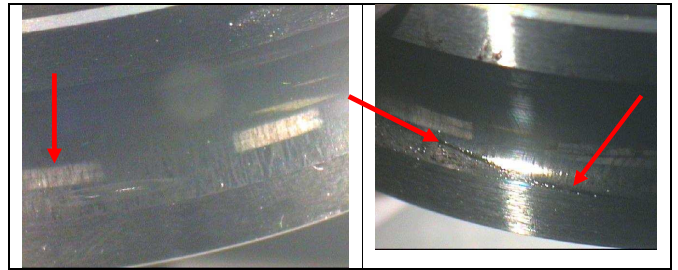
Figure 11: Left: Ball groove showing marks on ball track. Right: raceway, showing discoloured oil
