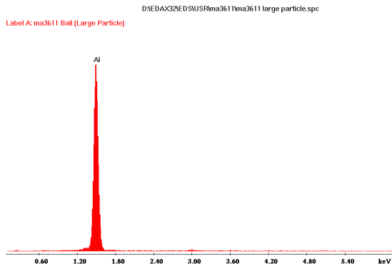
Figure 14: EDAX spectrum from metallic particle on ball showing Al-peak
