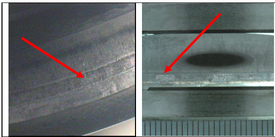
Figure 10: Inner raceway showing ball track
