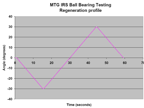
Figure 2: Regeneration profile used in life test programme
