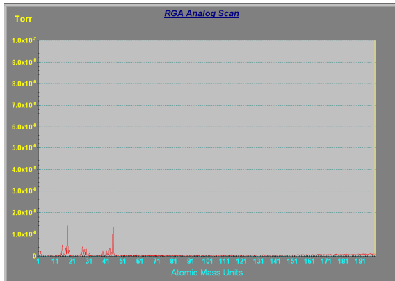
Figure 16: End of test, 20 deg C
