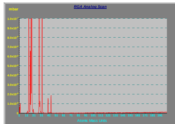
Figure 15: Start of testing (room temperature)
