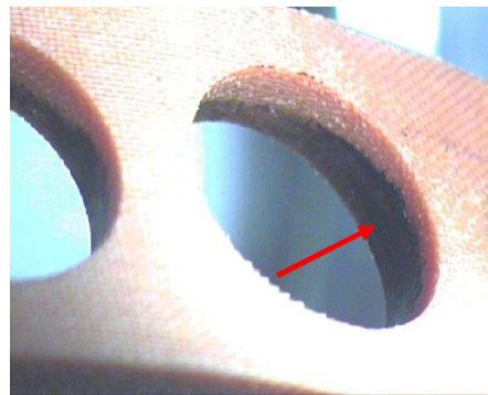
Figure 12: Darkened patch in ball pocket
