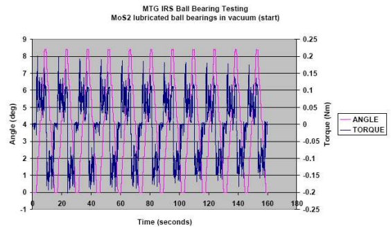
Figure 7: Baseline life test profile for \text{MoS}_2 lubricated ball bearings in vacuum
