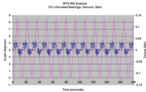
Figure 8: Baseline life test profile for oil lubricated ball bearings in vacuum
