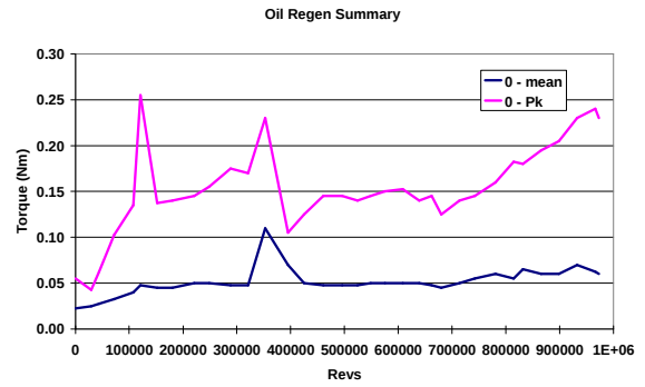
Figure 6: Summary of mean and 0-peak torques during regeneration cycles
