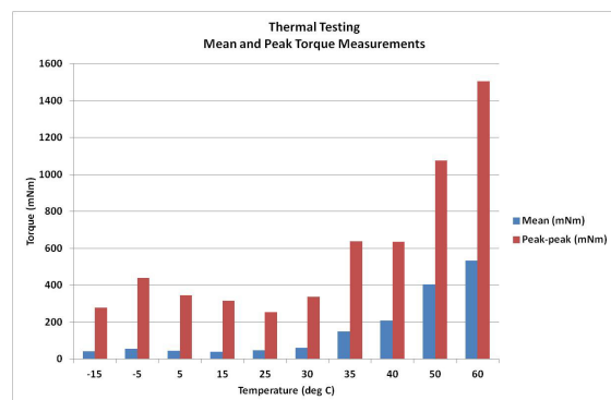
Figure 9: Results from thermal testing
