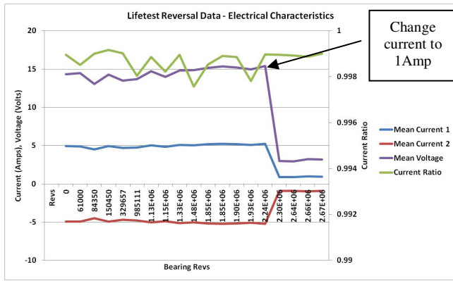
Figure 6: Summary of electrical data from torque reversals
