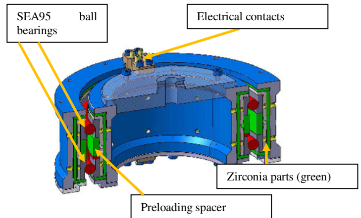
Figure 1: AGSM BBM2 – 3-D cross-section
