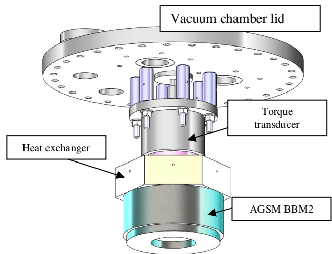
Figure 4: Test set-up
