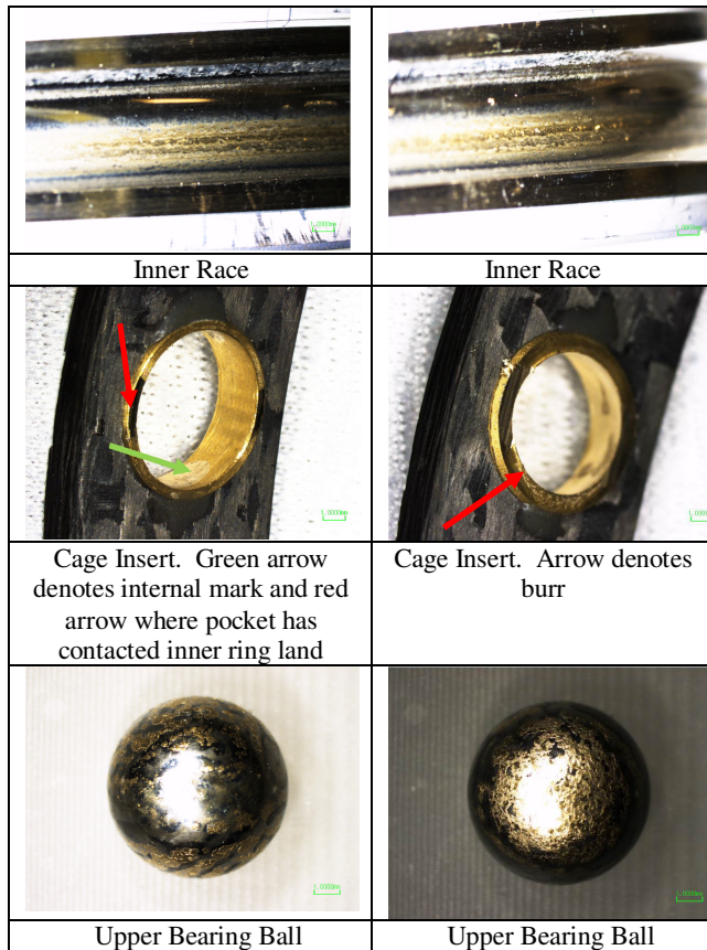
Figure 10: Upper Bearing Inspection
