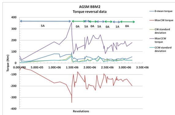
Figure 7: Summary of torques measured during reversals
