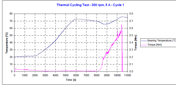
Figure 2: Torque increase above 50 deg C during testing at RUAG
