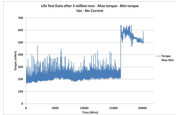
Figure 8: Torque increase at 3.2 million revs
