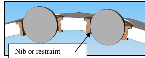
Figure 3: Schematic diagram showing design of cage inserts
