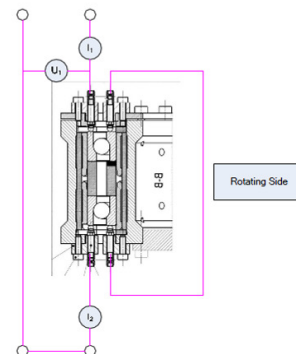
Figure 5: Electrical connections to ball bearing.
