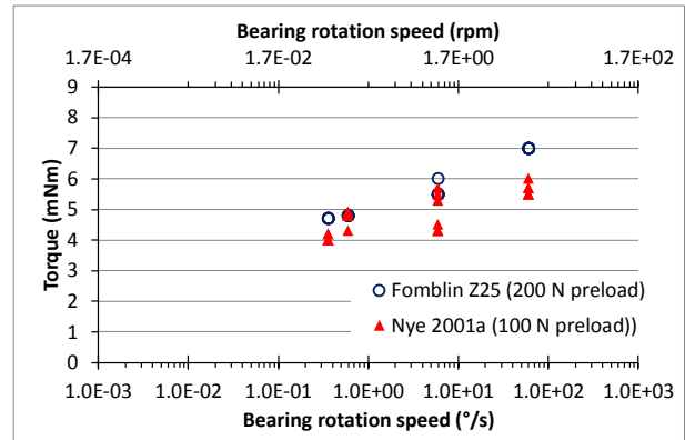
Figure 5. Oil lubrication mean torque. Test Programme 1.
