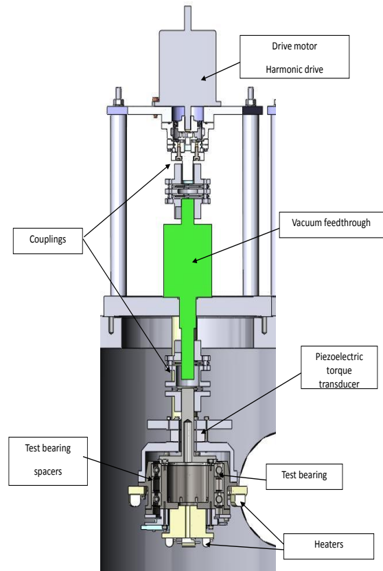
Figure 3. Bearing torque test rig. (Test Programme 2)
