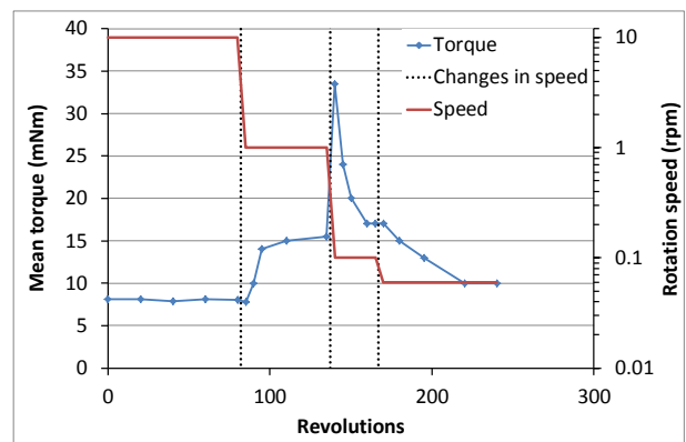
Figure 12. Series of tests of Braycote 601EF micronic. Test programme 1. 100 N hard preload.
