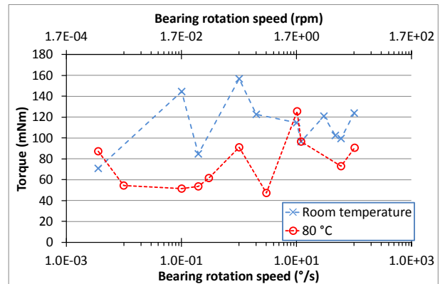
(a) Highest mean torque at each speed.
