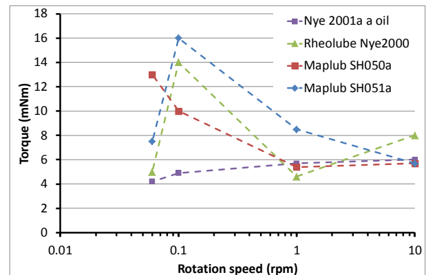
(b) Nye 2001a based lubricants, 100 N preload.
