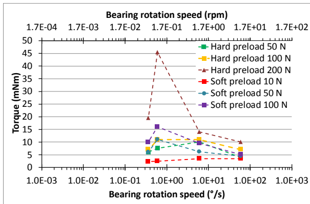
Figure 10. Grease lubrication mean torque, Test Programme 1, Braycote 601EF, various preload settings.
