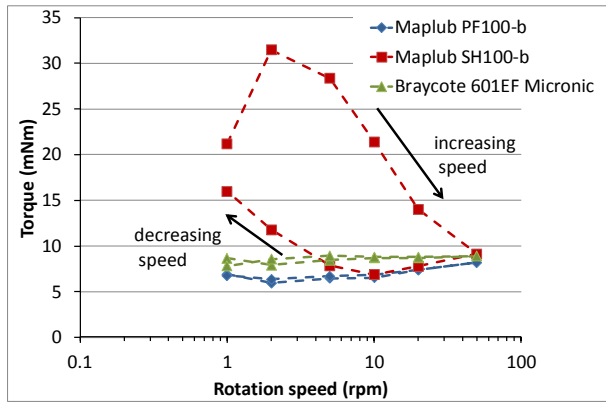
Figure 13. Tests of grease-lubricated angular contact, ball bearings (Barden type 104HC, 320 N preload) at speeds 1 to 50 rpm).
