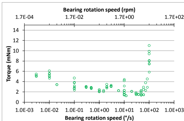
Figure 8. Standard deviation of torque. Test Programme 2. Nye 2001a, 1200 N preload.
