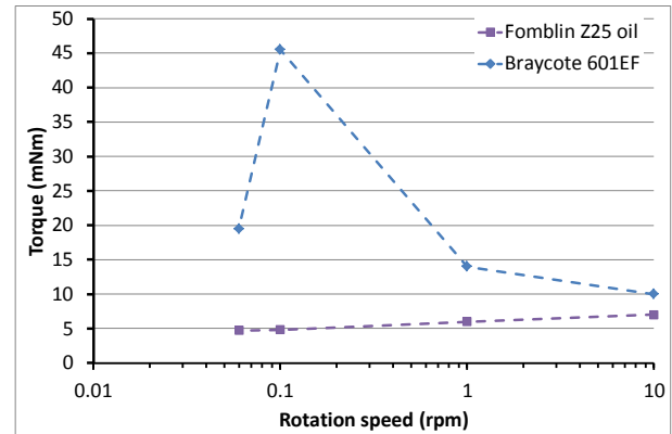
(a) Fomblin Z25-based lubricants, 200 N preload.
