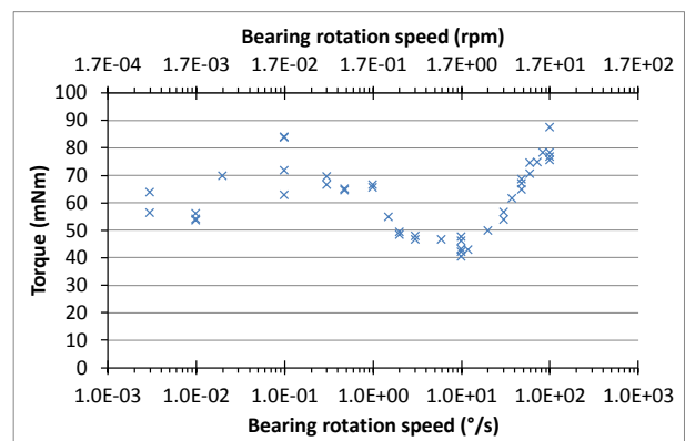
Figure 6. Oil lubrication mean torque. (Test Programme 2) Nye 2001a, 1200 N preload.
