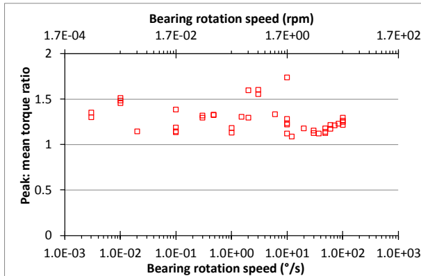
Figure 7. Peak-mean torque ratio. Test Programme 2. Nye 2001a, 1200 N preload.
