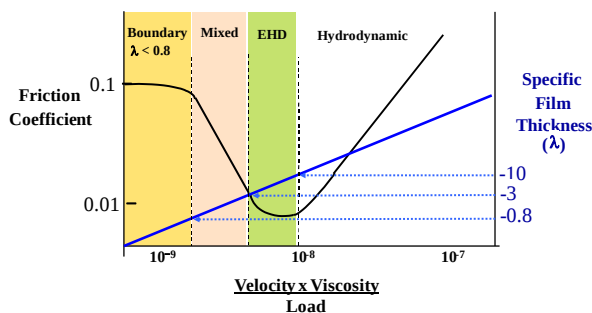
Fig.1 Stribeck curve: illustrating the various lubrication regimes for oil-lubricated contacts
