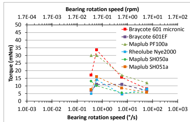
Figure 9. Grease lubrication mean torque, Test Programme 1, 100 N hard preload, range of greases.
