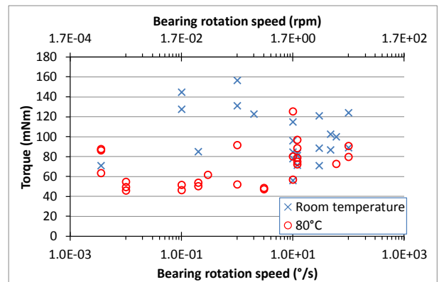
(b) All test results.
