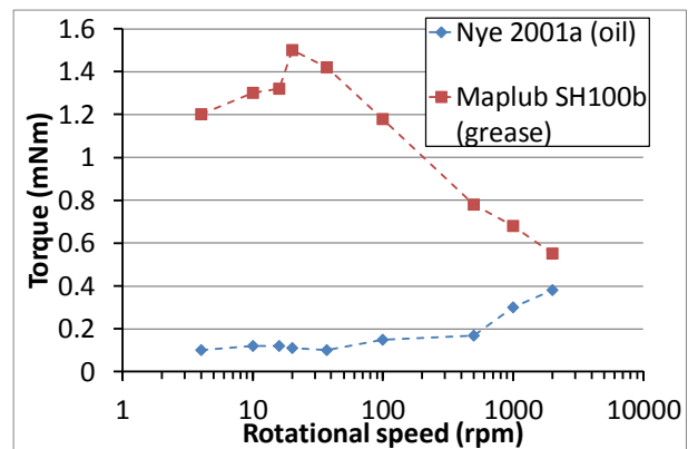
Figure 2. Showing torque vs. speed characteristics for SR4 bearing pair lubricated with SH100b grease and Nye2001a oil. 10 N preload, tests at 85°C [3].
