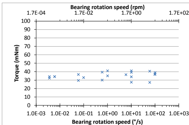
Figure 4. Solid lubrication mean torque. \text{MoS}_2 lubrication, 500 N preload (Test programme 2).
