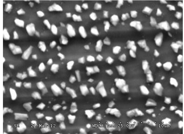
Figure 4. SEM image of 0.10 \mu\text{m} indium thin-film on 52100 steel disc.
