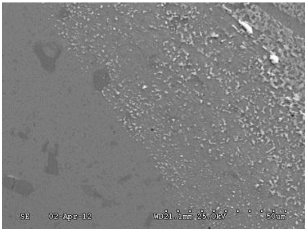
Figure 9. Edge of running track on SOT plate, showing a layer of transferred indium.
