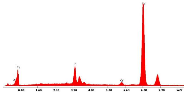
Figure 5. EDAX spectrum of 0.10 \mu\text{m} indium thin-film on 52100 steel disc.
