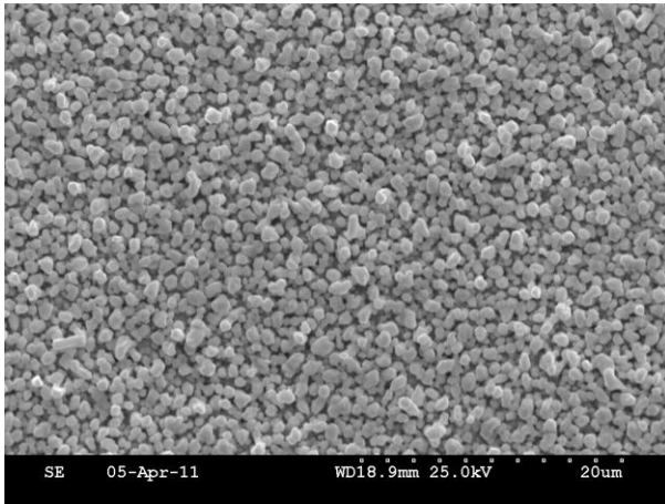
Figure 3. SEM image of 1 \mu m lead thin-film on 52100 steel disc.
