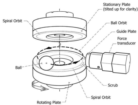
Figure 8. Internal arrangement of SOT.
