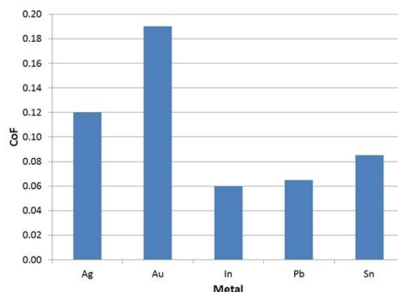
Figure 1. Friction coefficients of soft metal films in vacuum at room temperature (pin Si 3 N 4 , disc 440C, load 10N, speed 24mm/s) [3].
