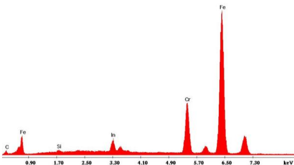
Figure 10. EDAX spectrum of running track on SOT plate, with clear indium signal. No indium peak was observed in a 'control' scan outside the running track.
