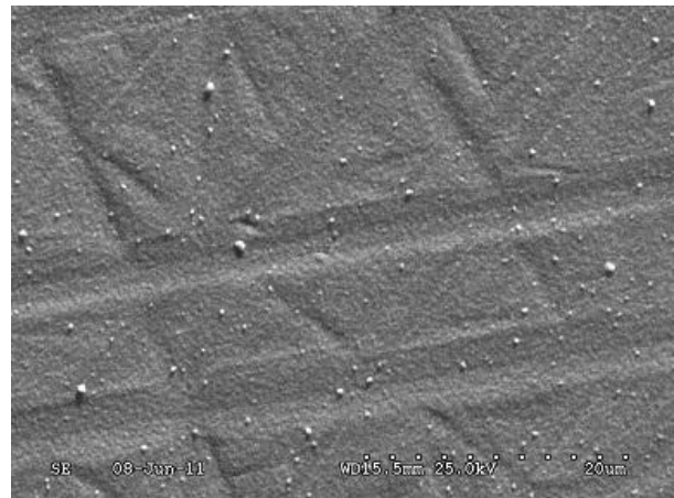
Figure 2. SEM image of 0.1µm lead thin-film on 52100 steel disc.
