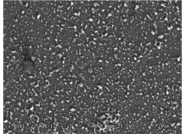
Figure 6. SEM image of 0.08µm indium thin-film on 52100 steel ball.
