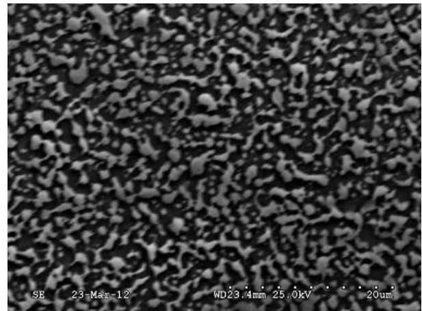
Figure 7. SEM image of 0.11µm indium thin-film on 52100 steel ball. Coating was produced without biasing the substrate.
