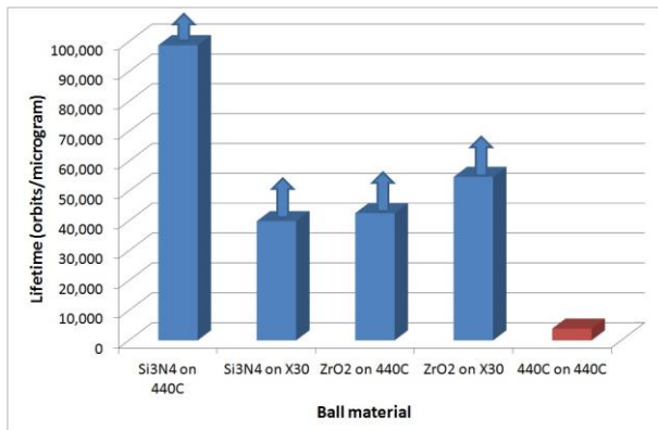
Figure 4. Normalised lifetimes of 2001a lubricated ceramic balls, in comparison to steel-on-steel [1]
