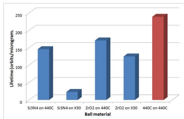
Figure 3. Normalised lifetimes of Z25 lubricated ceramic balls, in comparison to steel-on-steel [1]
