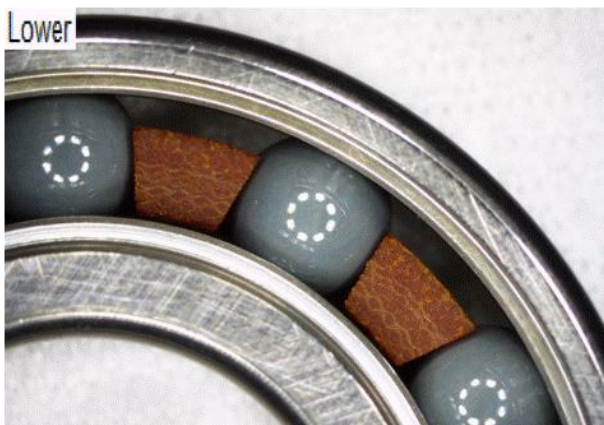
Figure 10. Test ID 3.2 lower bearing. Good condition, little sign of wear, oil transferred from cage to balls and races
