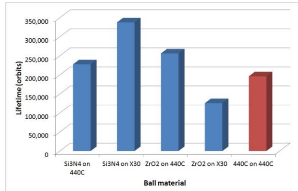
Figure 6. Normalised lifetimes of MoS 2 lubricated ceramic balls, in comparison to steel-on-steel [1]
