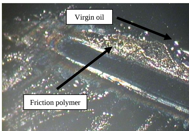
Figure 5. Guide plate from Test ID 2.5, showing polymer and virgin oil
