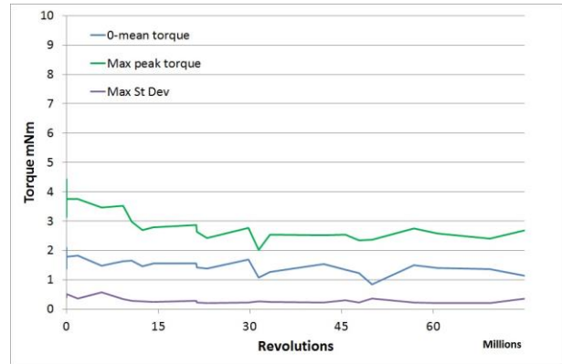
Figure 8. Test ID 3.1 torque progression (based on 2RPM reversals)
