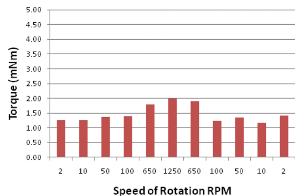
Figure 9. Pre-test variable speed testing for Test ID 3.1 bearing pair
