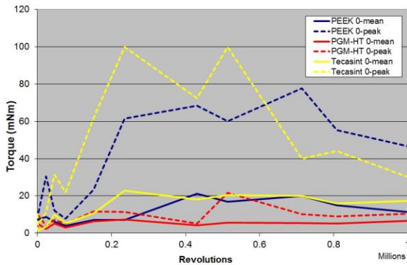
Figure 12. Torque progression of unlubricated ceramic bearings. Extremely high torques for PEEK and Tecasint 1391 were observed
