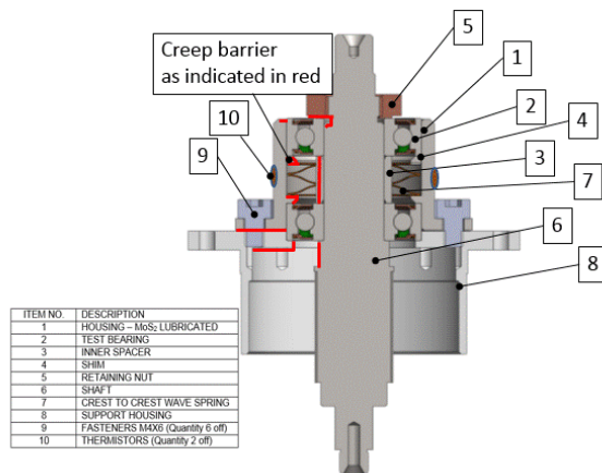
Figure 7. Schematic of test housing, showing location of creep barrier
