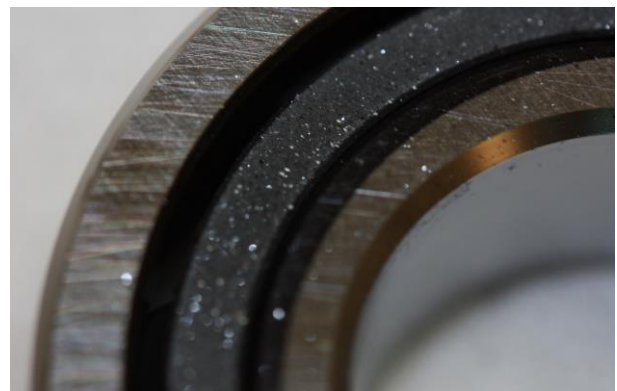
Figure 14. Dusting of \text{MoS}_2 debris visible on bearing lands and cage following 35-million revolution life-test
