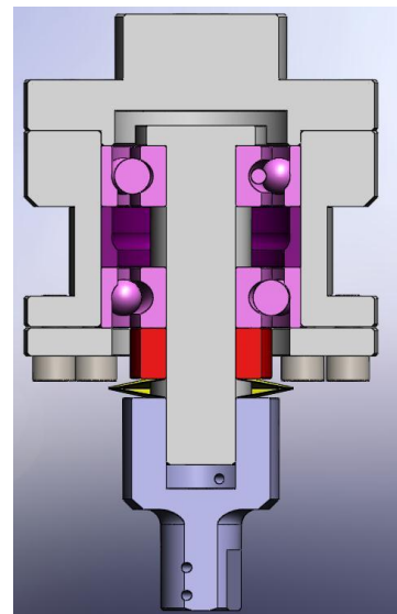
Figure 11. Bearing housing for B7004 bearing pairs, used during phase four
