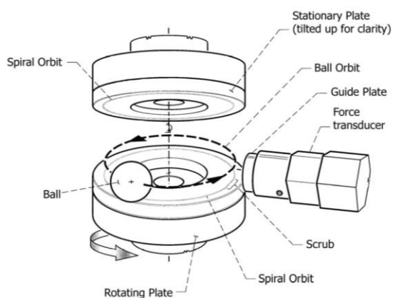
Figure 2. Internal arrangement of SOT
