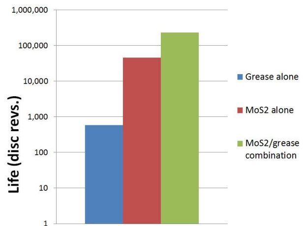
Figure 11. Mean lifetimes for Braycote 601EF and MoS 2 , separately and in combination, during phase three of testing
