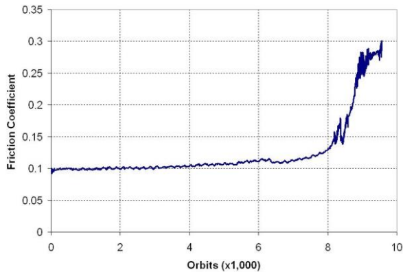
Figure 8. Example friction trace of Fomblin Z25 in vacuum [9]
