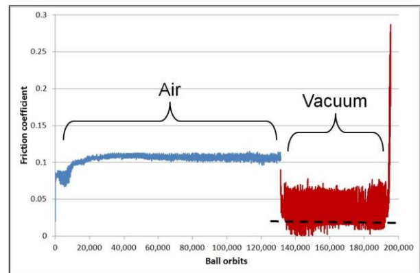
Figure 4. Z25/MoS 2 rolling in air (blue) and vacuum (red). Dashed line shows the true vacuum friction
