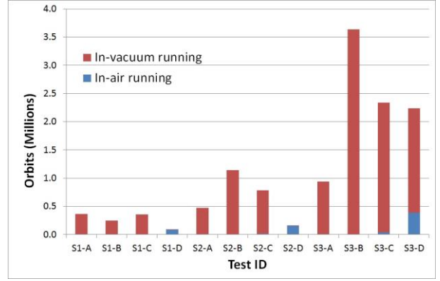
Figure 6. Rolling lifetime of phase two SOT tests
