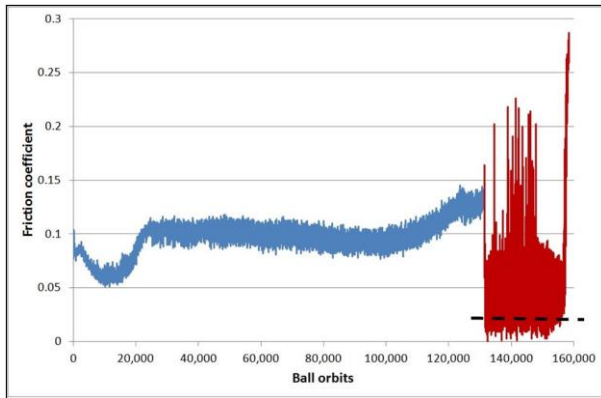
Figure 5. Synalox/MoS 2 rolling in air (blue) and vacuum (red).
