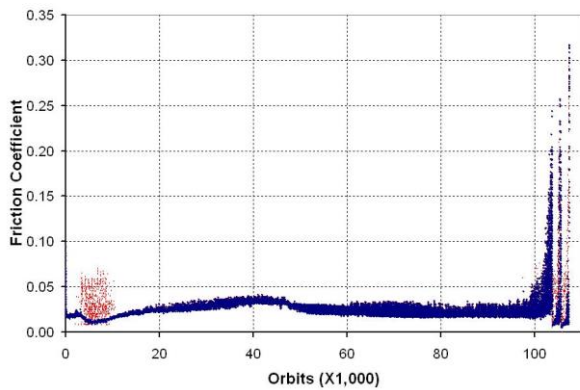
Figure 9. Example friction trace of sputtered MoS 2 in vacuum [9]
