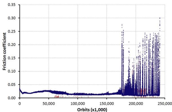
Figure 10. Friction trace from in-vacuo stage of S1-B,
