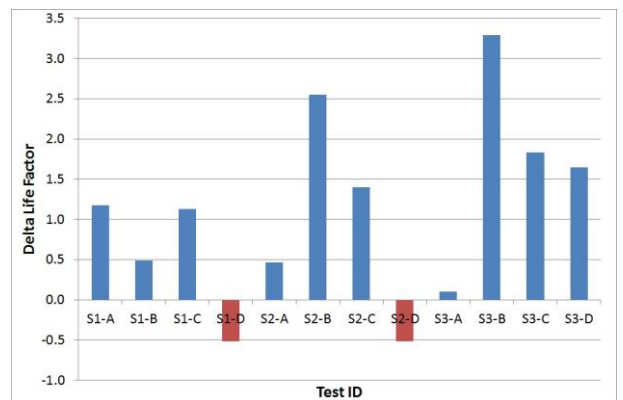
Figure 7. Delta-life extensions of 'hybrid' lubrication in comparison to predicted lifetime of the lubricant constituents
