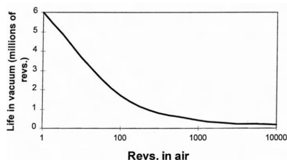
Figure 1. Low-torque life of \text{MoS}_2 lubricated ED20 bearings in vacuum as a function of the amount of in-air operation prior to vacuum tests [4]
