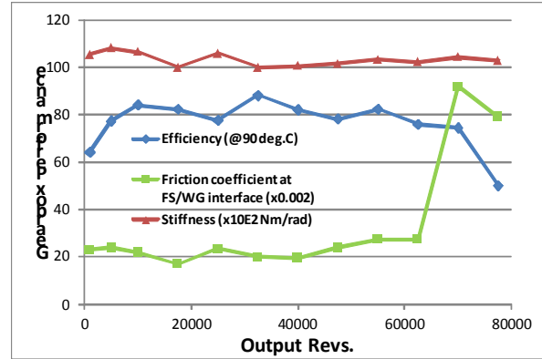
Figure 6. The evolution of efficiency, stiffness and FS/WG friction (at +90°C) during the endurance testing of a MAC-lubricated HFUC-20-160 Harmonic Drive® component set
