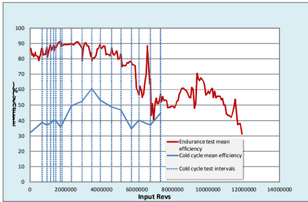
Figure 2. Evolution of efficiency of PFPE-lubricated gearbox (HFUC5) during endurance test.
