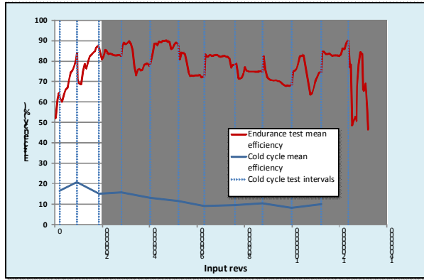
Figure 5. Evolution of efficiency of MAC-lubricated gearbox (HFUC7) during endurance test.
