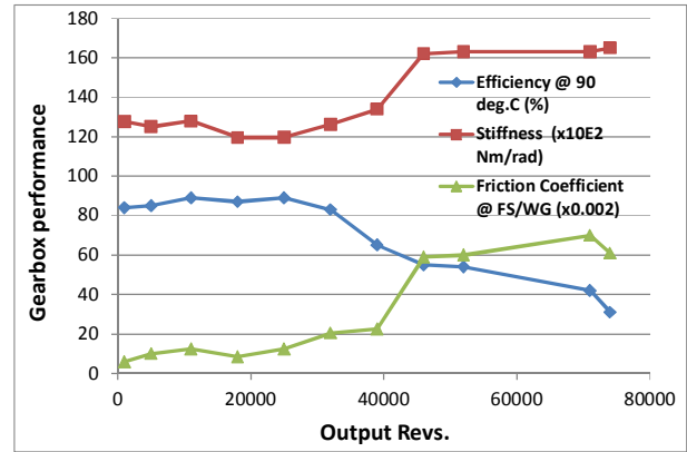
Figure 3. The evolution of efficiency, stiffness and FS/WG friction (at +90°C) during the endurance testing of a PFPE-lubricated HFUC-20-160 Harmonic Drive® component set.
