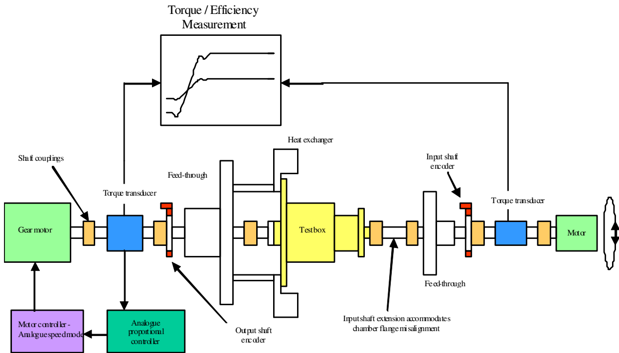
Figure 1. Schematic diagram of test rig
