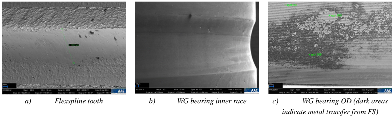
Figure 4. SEM micrographs of surface condition of gearbox (HFUC5) parts
