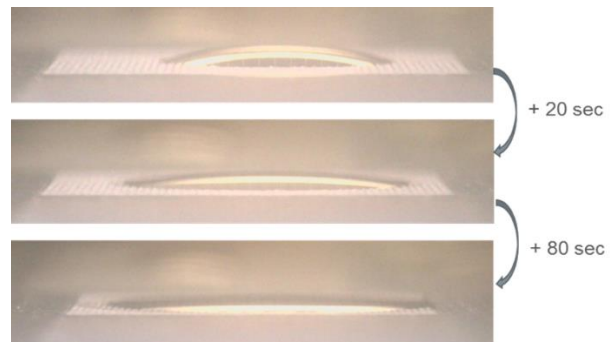
Figure 2. Lubricant mobility trials of cross-hatch LST microstructures
