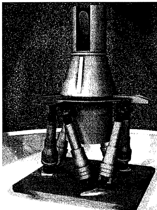
Figure 1. Hexapod / SAGE III layout.
