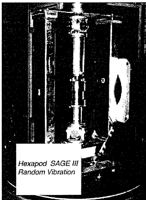
Figure 4. Random vibration test fixture.
