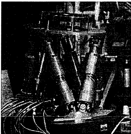
Figure 2. Hexapod Development Model.
