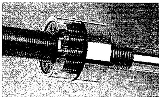
Figure 3. Satellite Roller screw sample.
