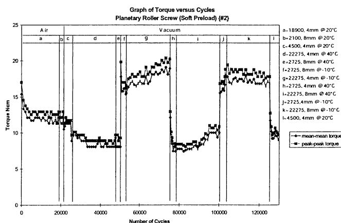
Figure 7. Torque vs cycles during thermo-vacuum test.
