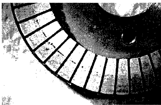
Figure 4 Piezomotor Segments After Successful Completion of Lifetest Showing Minor Evidence of Thermal Degradation.
