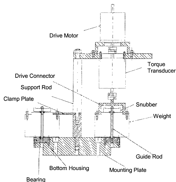
Figure 1 Test set-up for Torque and Vibration Test
