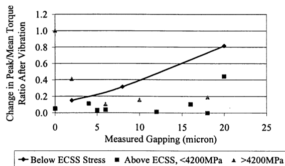
Figure 3 Changes in Torque noise from gapping
