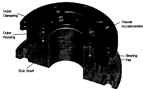
Figure 6 General Arrangement of Test set-up
