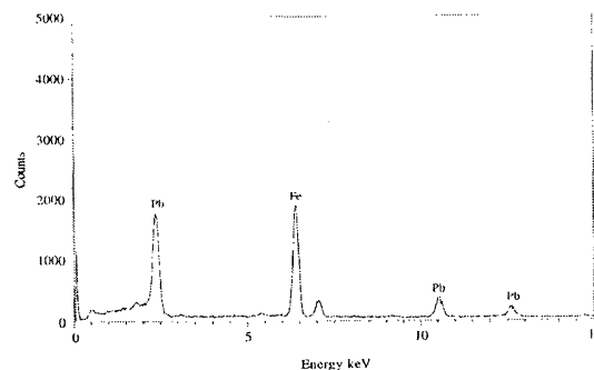
Figure 9 Energy Disperse X-ray Profile of Raceway of Figure 7 Non-Vibration-affected Zone
