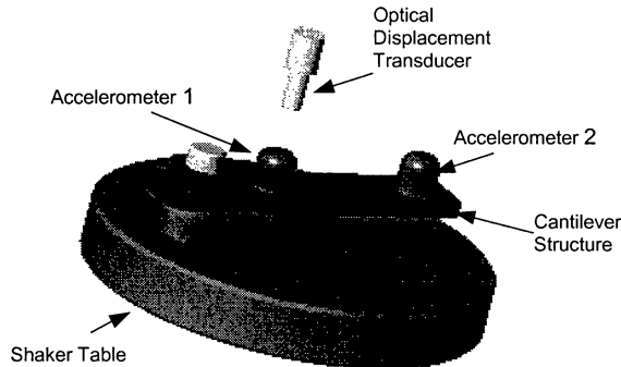
Figure 4 Test set-up for Verification of Displacement Measurement
