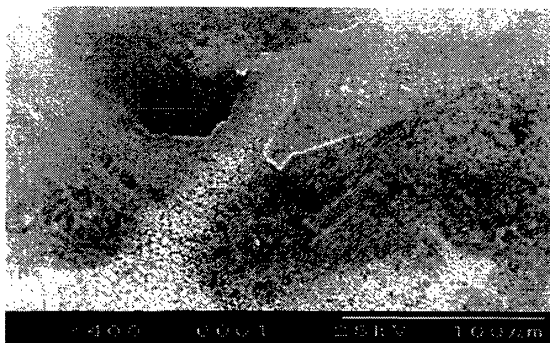
Figure 8 Scanning Electron Micrograph of the Edge of elliptical Zone of Lead lubricated Raceway shown in Figure 7
