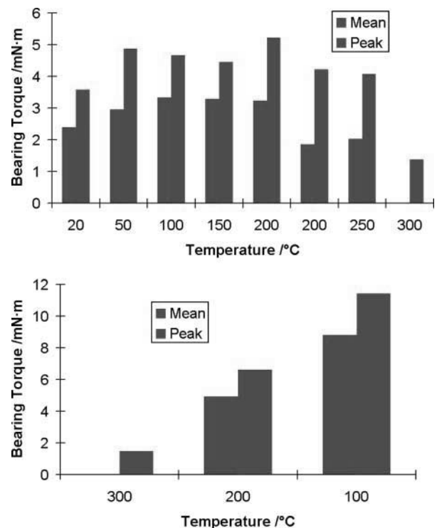
Fig. 5 Results of initial tests of MoS 2 -lubricated bearings with PGM-HT cages: (a) initial torque variation with increase in temperature and (b) decrease in temperature
