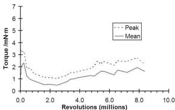
Fig. 7 Life test of MoS 2 -lubricated bearings with PGM-HT cages with cuts
