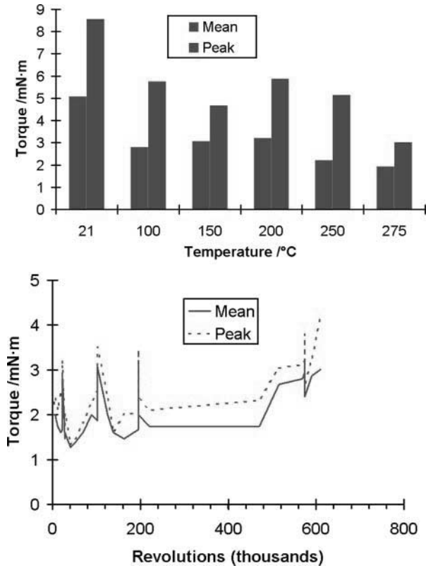
Fig. 11 Results from the test of full titanium cage: (a) initial torque variation with temperature and (b) life test at 200 r/min
