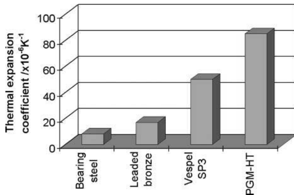
Fig. 1 Thermal expansion coefficients of self-lubricating bearing cage materials
