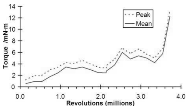
Fig. 4 Results of life tests of lead-lubricated bearings with leaded bronze cages
