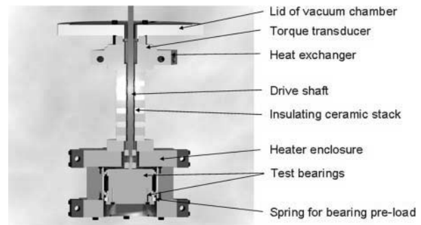
Fig. 2 High-temperature bearing test rig
