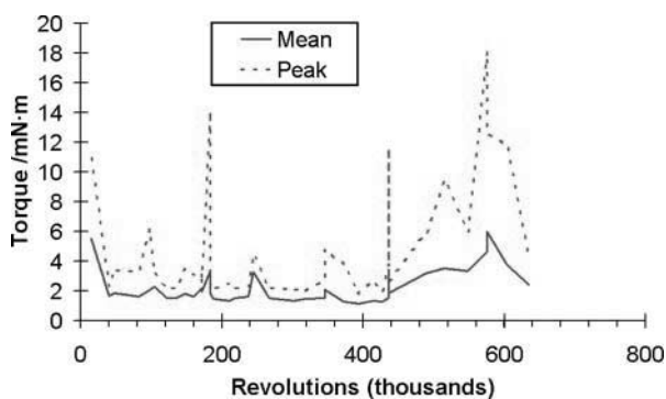
Fig. 13 Results from the life test of hybrid cage with SINTIMID 15M-HT inserts, without lubricant coating on balls and races
