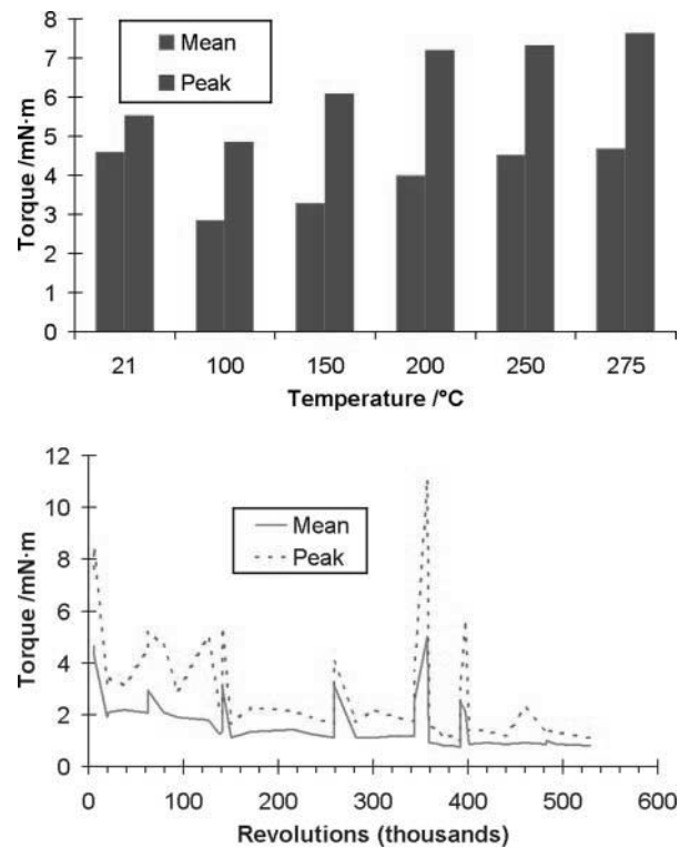
Fig. 14 Results from the test of hybrid cage with PGM-HT inserts, with MoS 2 coating on balls and races: (a) initial torque variation with temperature and (b) life test at 200 r/min
