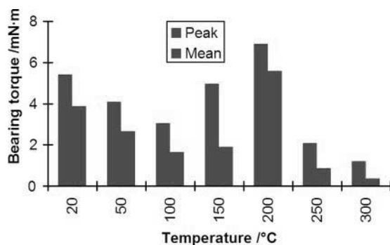
Fig. 6 Repeat tests of MoS 2 -lubricated bearings with PGM-HT cages with cuts – torque measurements at various temperatures
