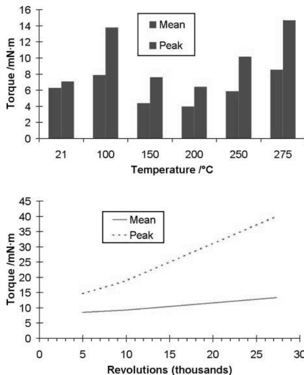
Fig. 17 Results from the test of PTFE toroids, with MoS 2 coating on balls and races: (a) initial torque variation with temperature and (b) life test at 200 r/min
