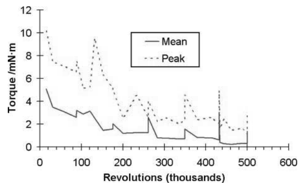
Fig. 15 Results from the life test of hybrid cage with PGM-HT inserts, without lubricant coating on balls and races
