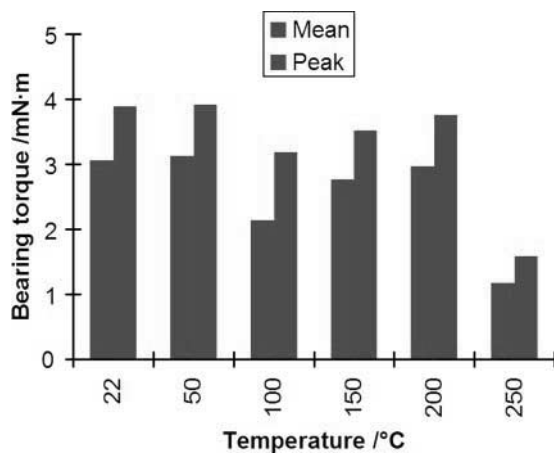
Fig. 3 Results of initial tests of lead-lubricated bearings with leaded bronze cages
