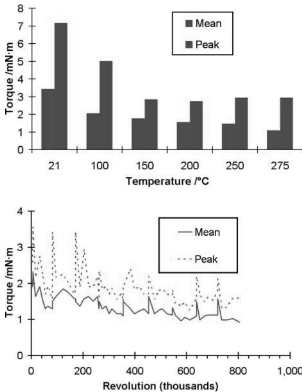
Fig. 12 Results from the test of hybrid cage with SINTIMID 15M-HT inserts, with MoS 2 coating on balls and races: (a) initial torque variation with temperature and (b) life test at 200 r/min
