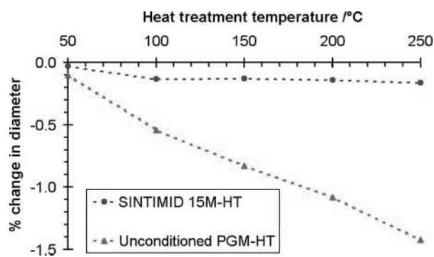
Fig. 8 Size variation of PGM-HT and SINTIMID 15M-HT 'dummy cages' after heating to a range of temperatures
