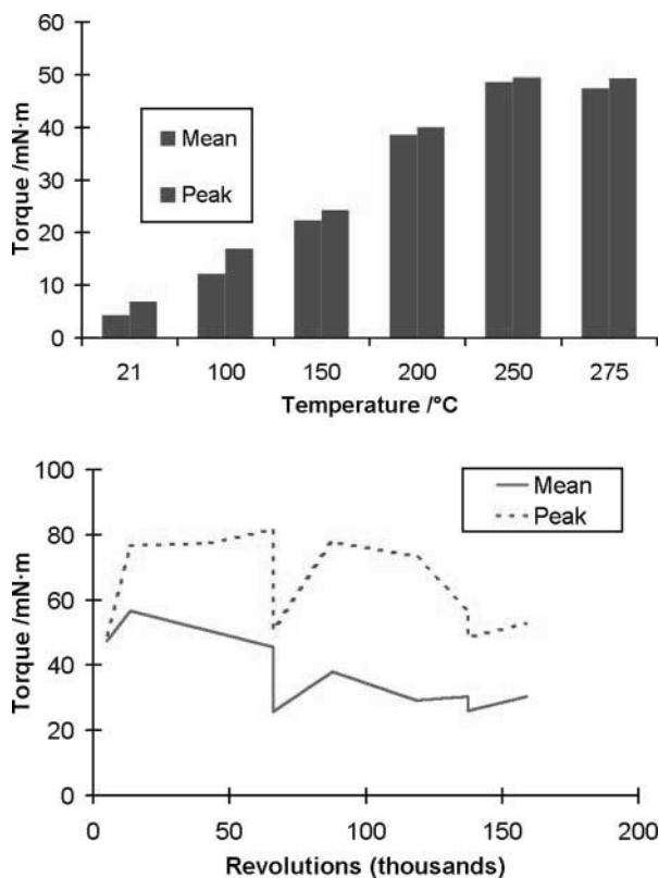
Fig. 16 Results from the test of PGM-HT toroids, with MoS 2 coating on balls and races: (a) initial torque variation with temperature and (b) life test at 200 r/min
