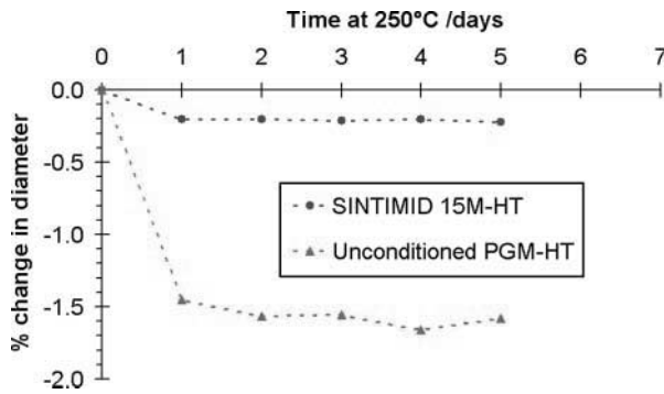
Fig. 9 Dimensional change of dummy cages after heating to 250 °C. Cages measured at room temperature after each 24 h heating period
