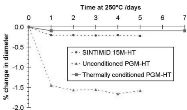
Fig. 10 Dimensional change of 'dummy cages' after heating to 250 °C
